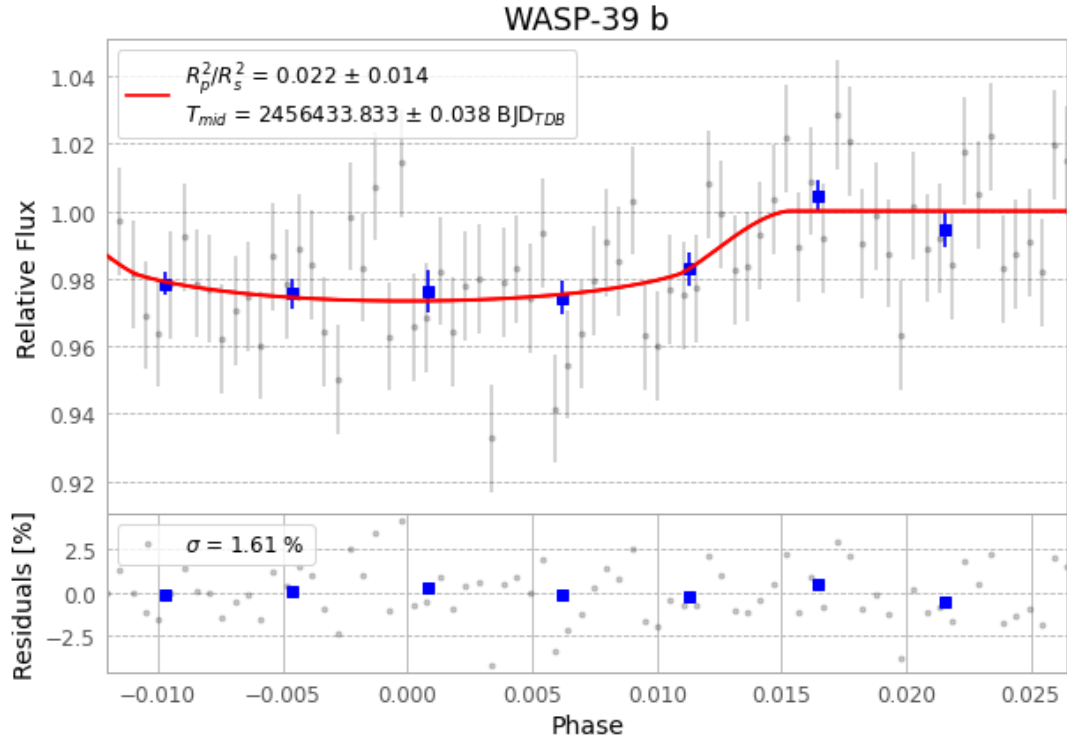
Figure 1 — FinalLightCurve_WASP-39 b_2013-05-20.png (SHA-256 1e21ca22f58c3fe2...)
