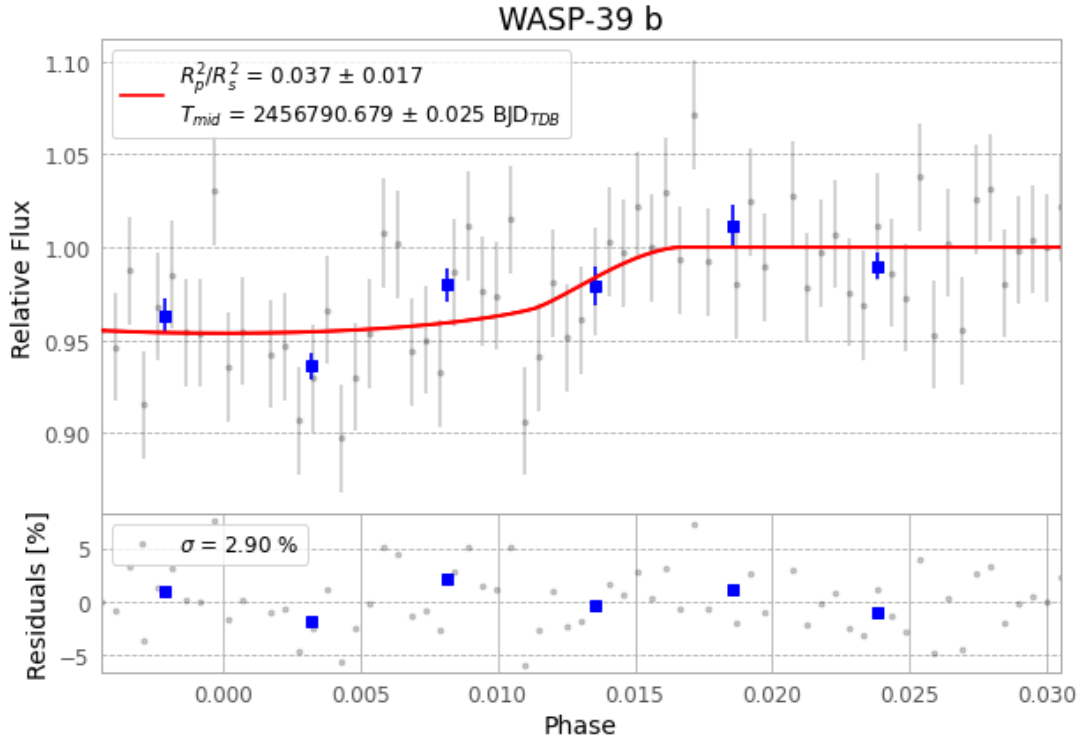
Figure 1 — FinalLightCurve_WASP-39 b_2014-05-12.png (SHA-256 4689ae2276d27b4c...)
