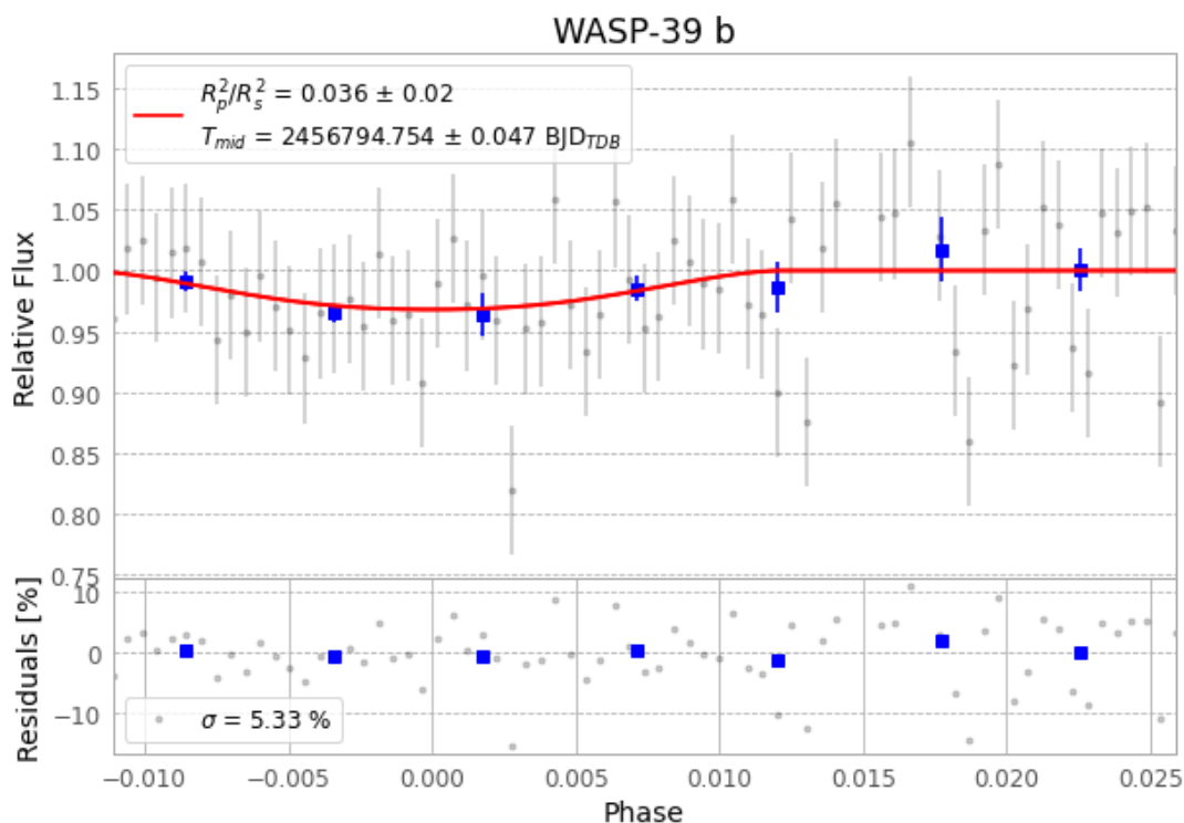
Figure 1 — FinalLightCurve_WASP-39 b_2014-05-16.png (SHA-256 d35d79114fe2872b...)
