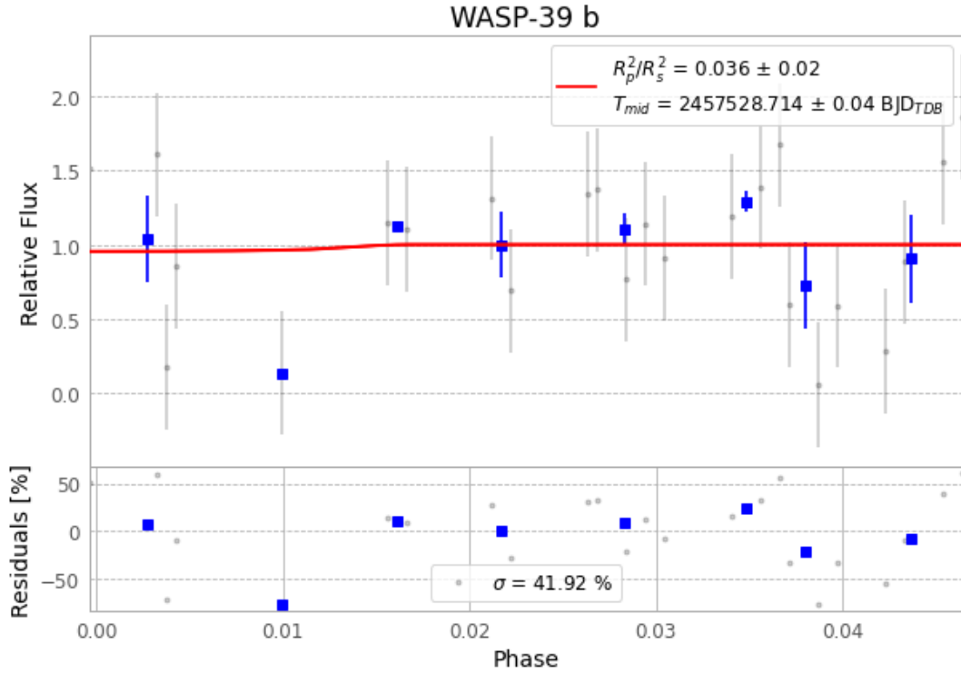
Figure 1 — FinalLightCurve_WASP-39 b_2016-05-19.png (SHA-256 015c76cea3bd44df...)
