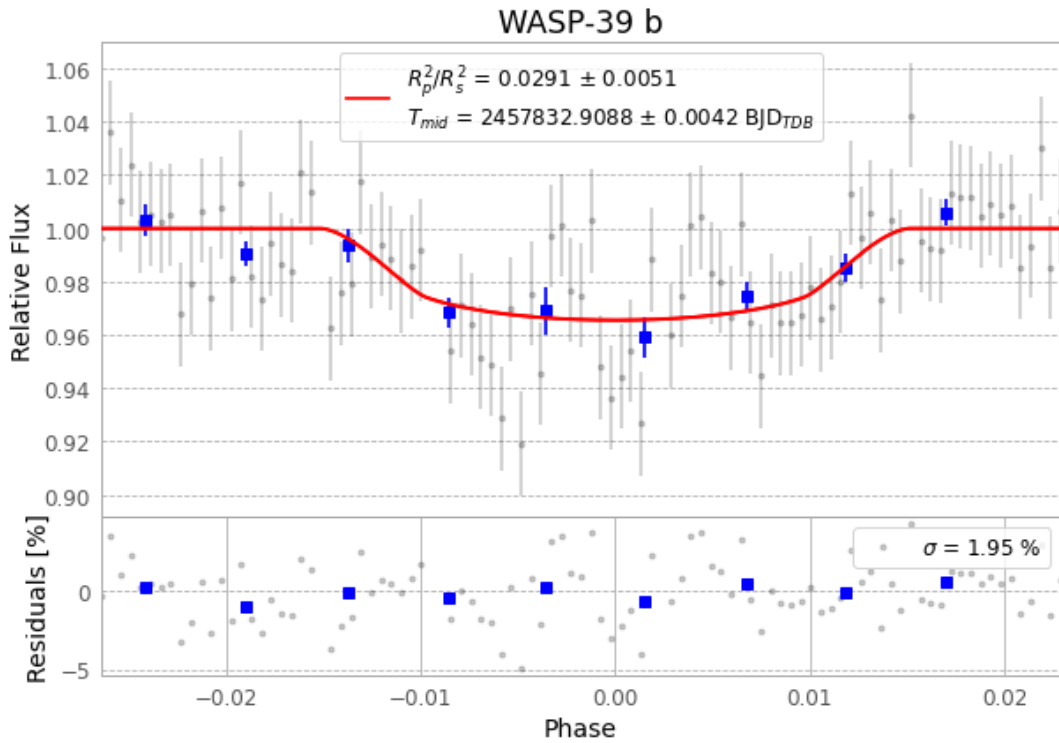
Figure 1 — FinalLightCurve_WASP-39 b_2017-03-20.png (SHA-256 d8542004a93d085b...)
