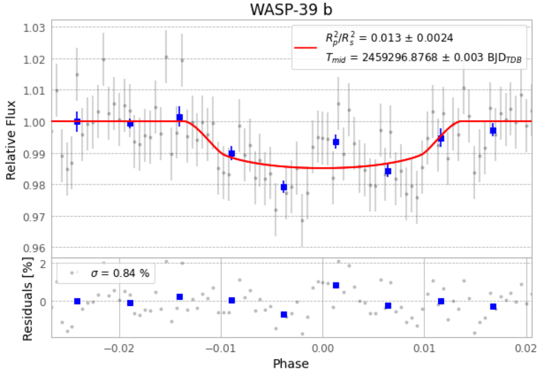
Figure 1 — FinalLightCurve_WASP-39 b_2021-03-22.png (SHA-256 d69d495387b94a13...)
