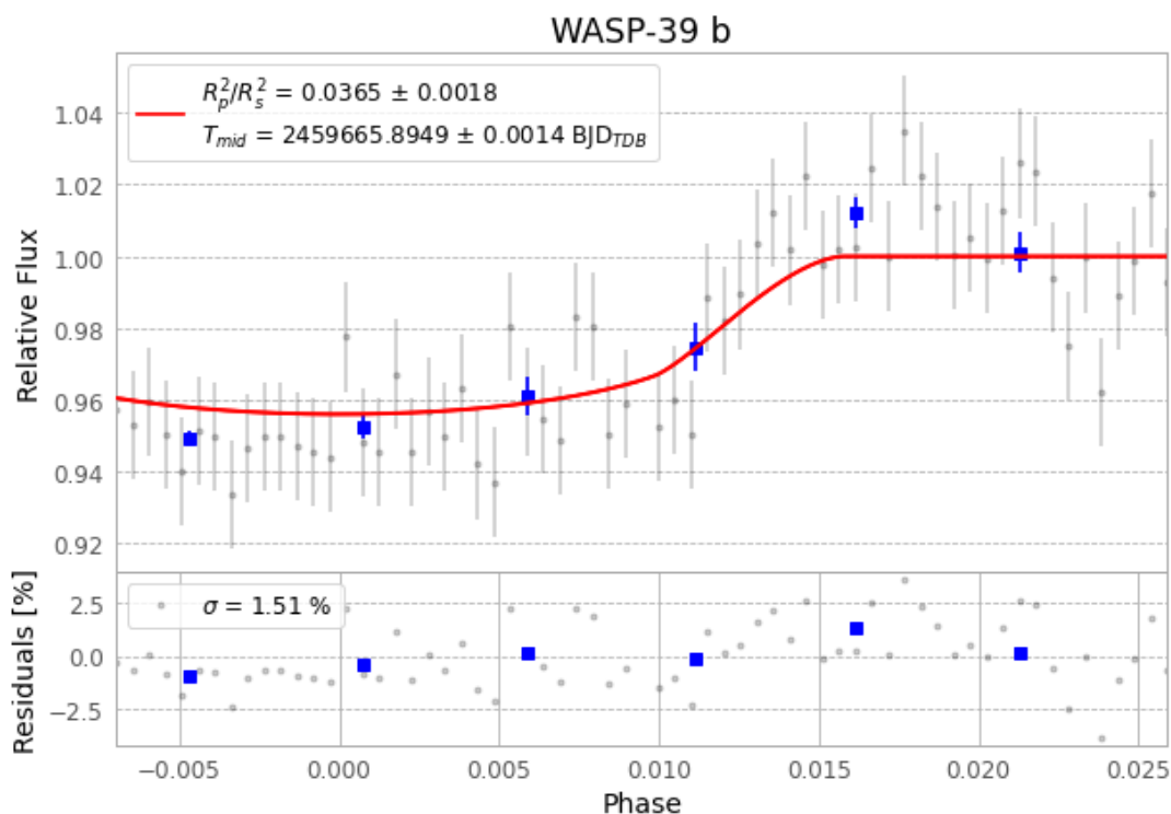
Figure 1 — FinalLightCurve_WASP-39 b_2022-03-27.png (SHA-256 19ebe0d5350d2369...)
