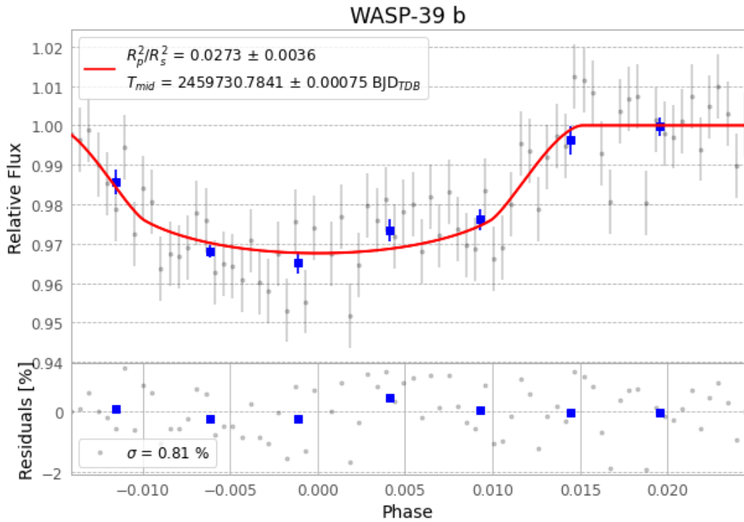
Figure 1 — FinalLightCurve_WASP-39 b_2022-05-30.png (SHA-256 5a81323d7723b646...)
