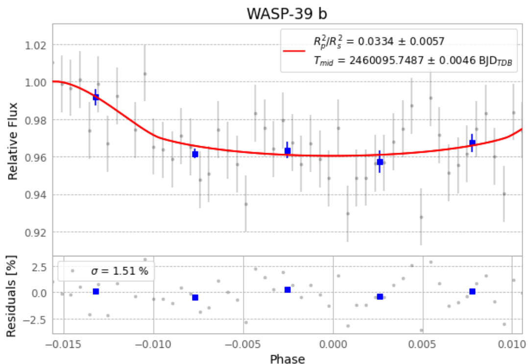
Figure 1 — FinalLightCurve_WASP-39 b_2023-05-30.png (SHA-256 825cb8e65442f35d...)
