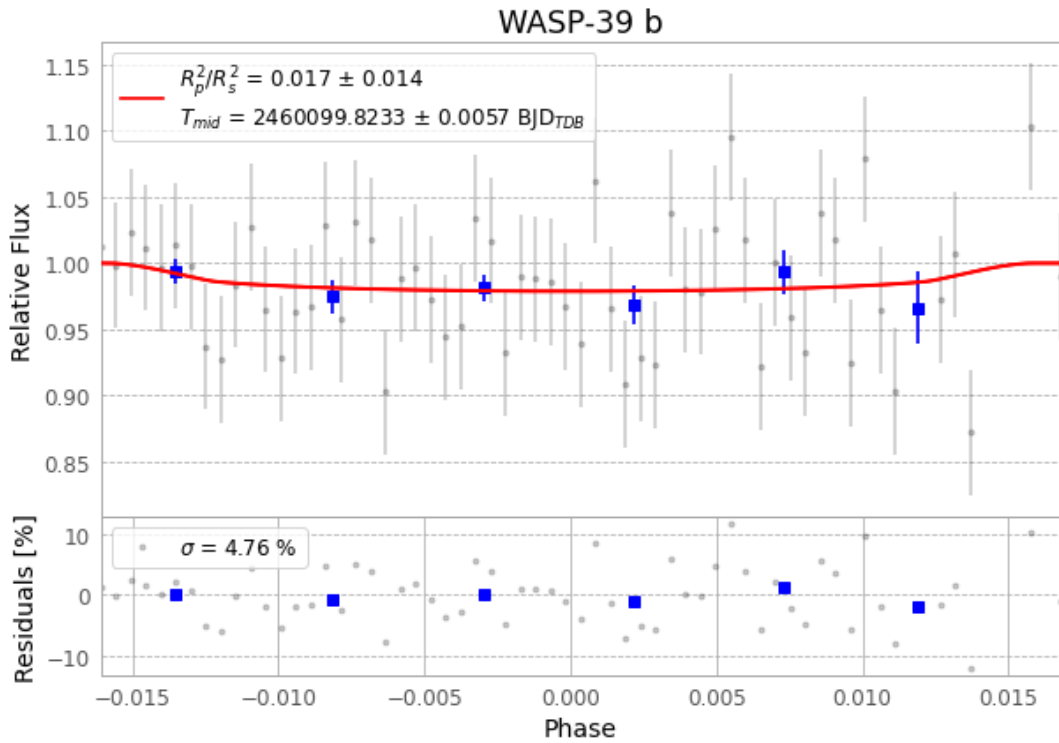
Figure 1 — FinalLightCurve_WASP-39 b_2023-06-03.png (SHA-256 d8f12baa48b39f9c...)
