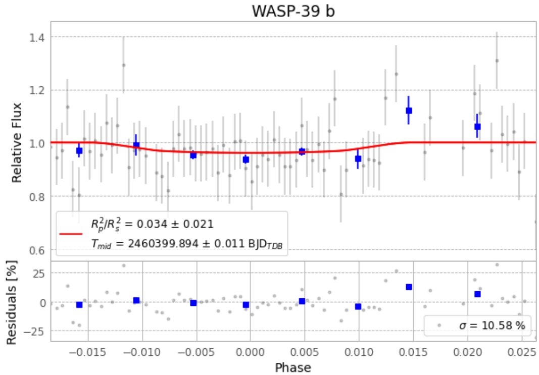
Figure 1 — FinalLightCurve_WASP-39 b_2024-03-30.png (SHA-256 e1f9a011383d1c19...)
