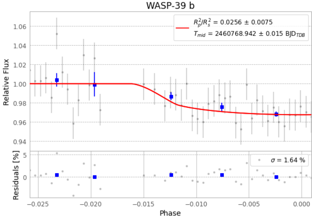
Figure 1 — FinalLightCurve_WASP-39 b_2025-04-03.png (SHA-256 c9fe5ae98447017...)
