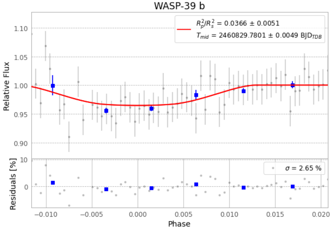
Figure 1 — FinalLightCurve_WASP-39 b_2025-06-02.png (SHA-256 118f0e0205d9e452...)
