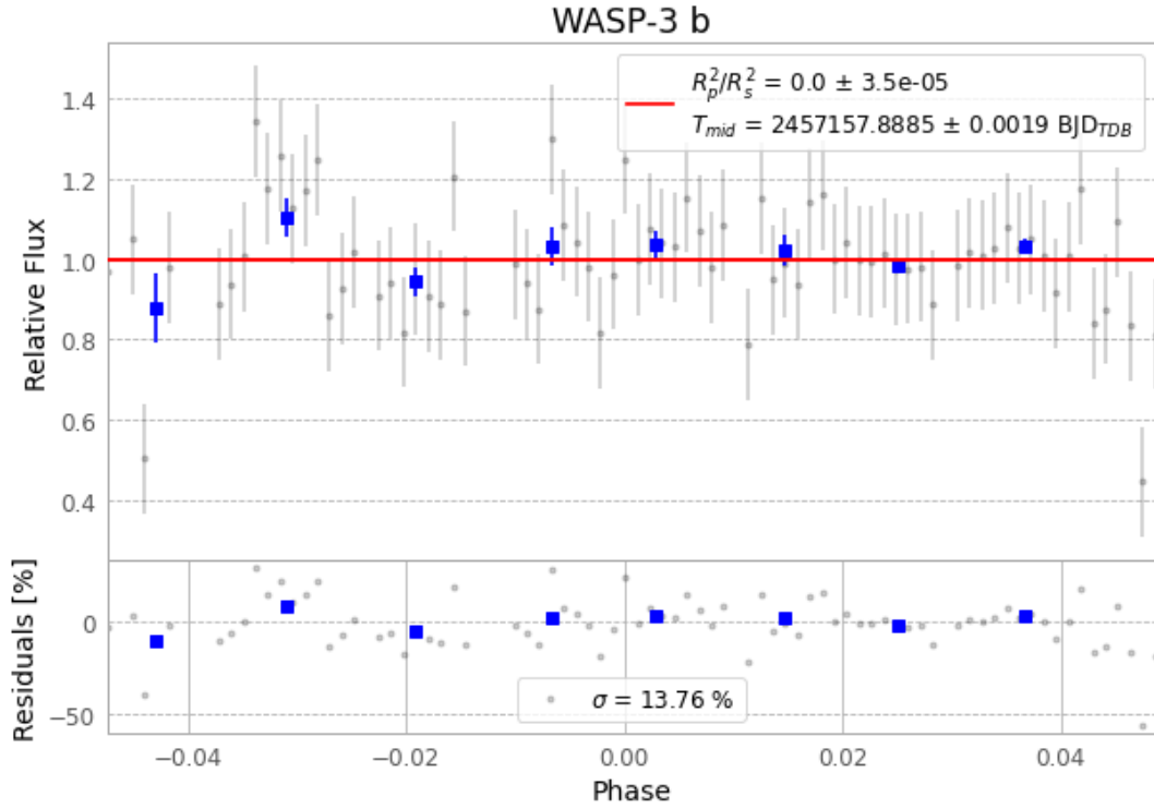
Figure 1 — FinalLightCurve_WASP-3 b_2015-05-15.png (SHA-256 584099f45255695f...)
