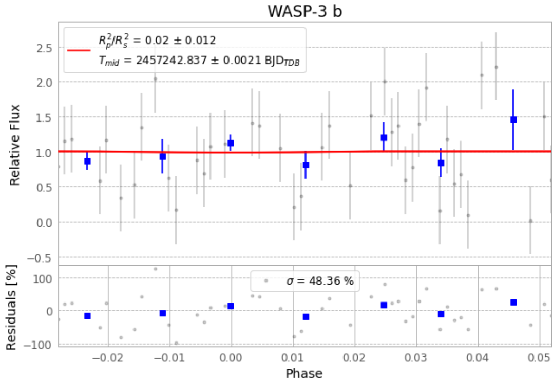
Figure 1 — FinalLightCurve_WASP-3 b_2015-08-07.png (SHA-256 27c6018382ed8446...)
