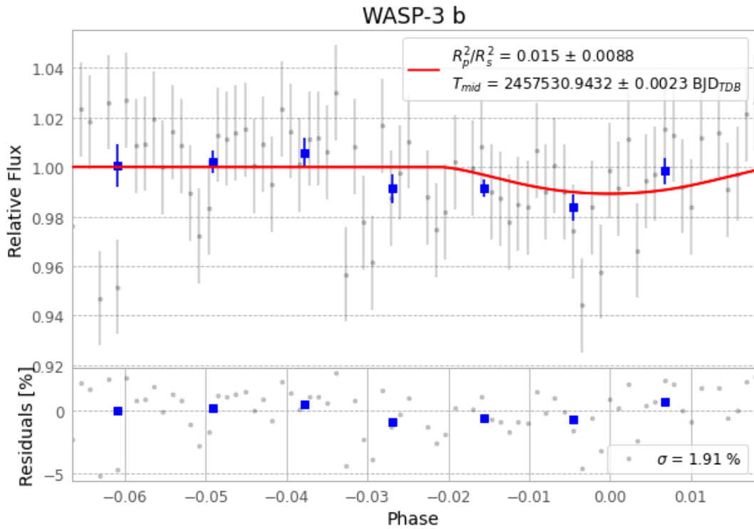
Figure 1 — FinalLightCurve_WASP-3 b_2016-05-22.png (SHA-256 1c2228c6f6b58fb3...)
