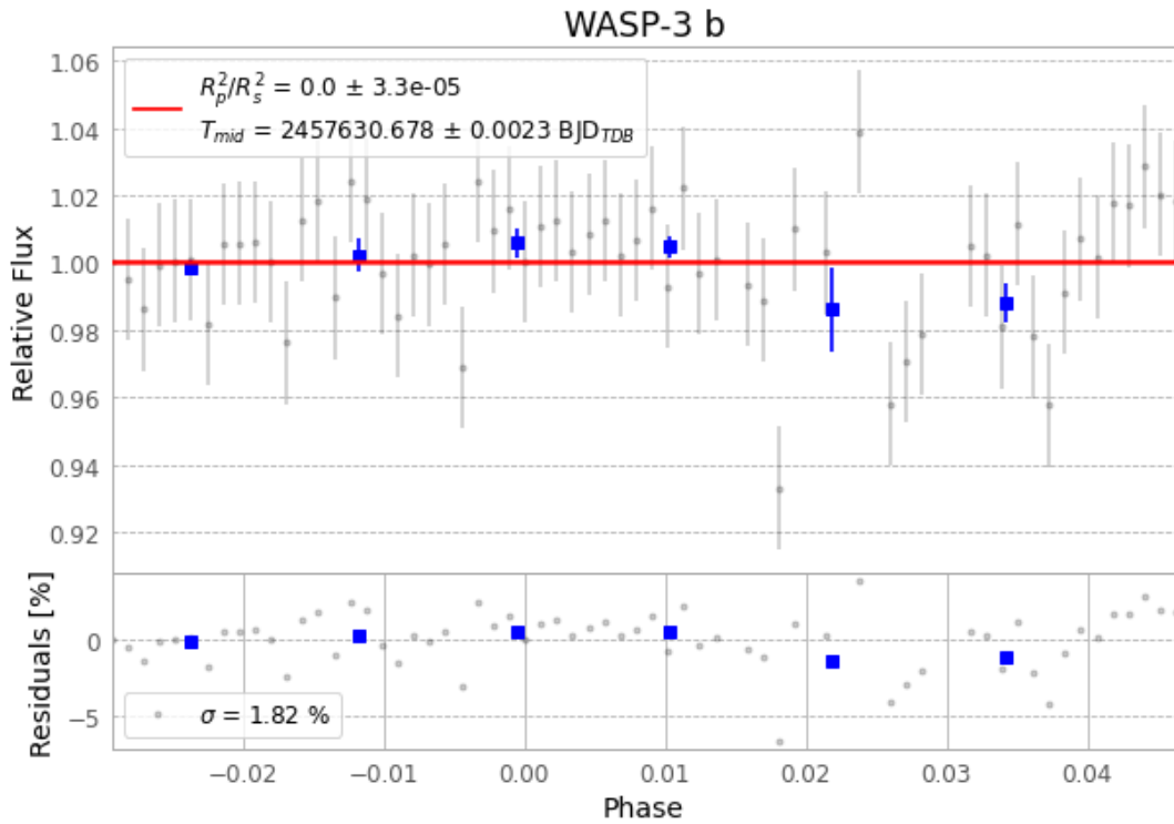
Figure 1 — FinalLightCurve_WASP-3 b_2016-08-29.png (SHA-256 e2f4b7ac8b19134f...)
