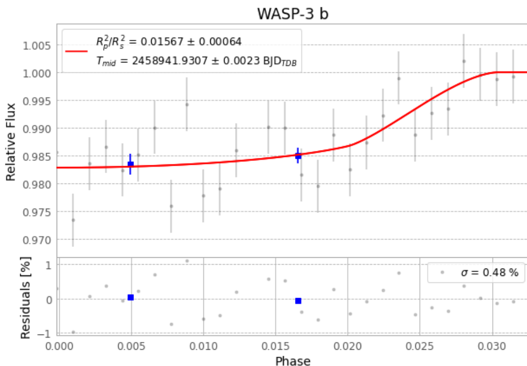
Figure 1 — FinalLightCurve_WASP-3 b_2020-04-02.png (SHA-256 6c5597951a8854e6...)
