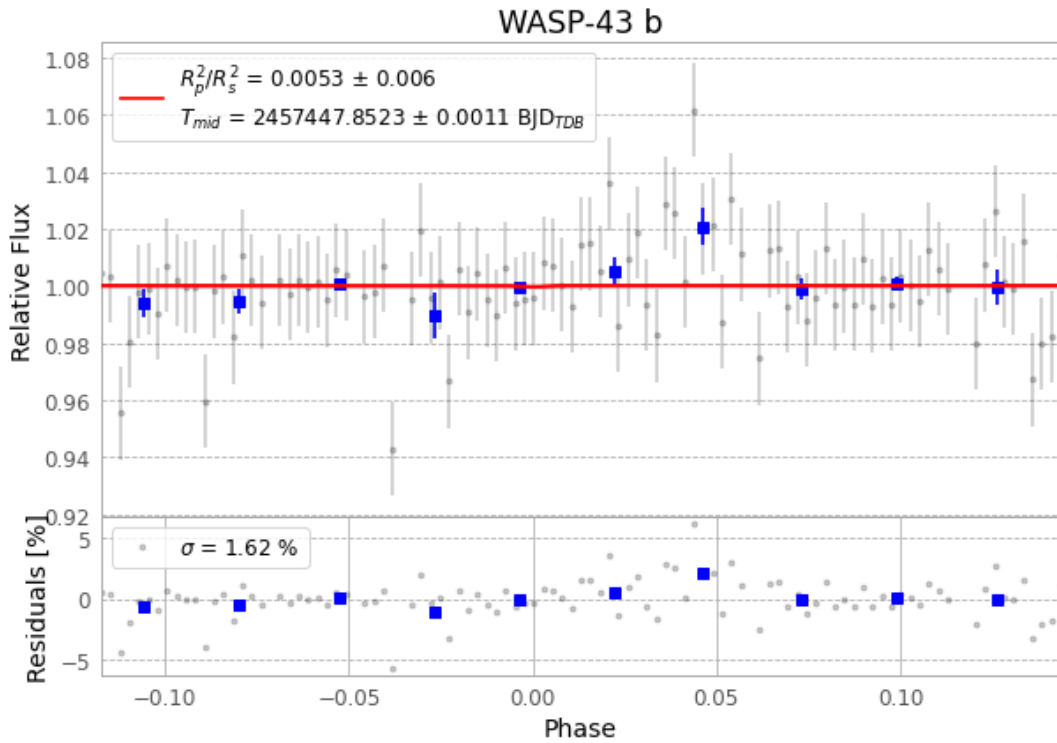
Figure 1 — FinalLightCurve_WASP-43 b_2016-02-28.png (SHA-256 f64f5645345f80a0...)
