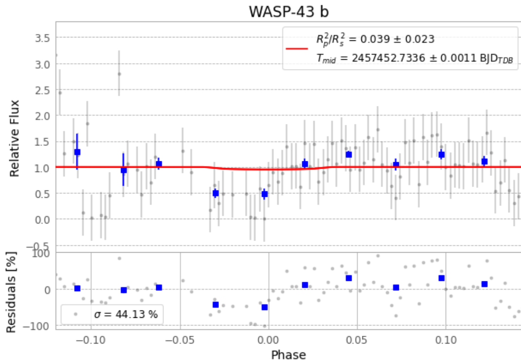
Figure 1 — FinalLightCurve_WASP-43 b_2016-03-04.png (SHA-256 6a679a6fb99c0c72...)
