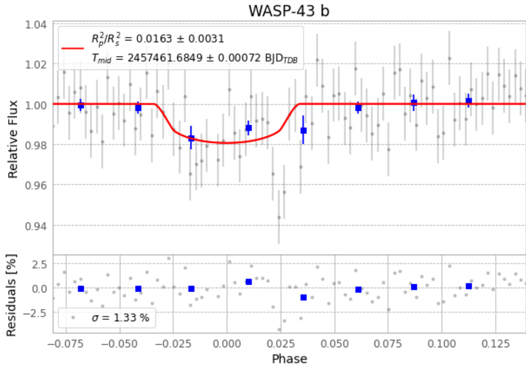
Figure 1 — FinalLightCurve_WASP-43 b_2016-03-13.png (SHA-256 418fc4798ef81392...)
