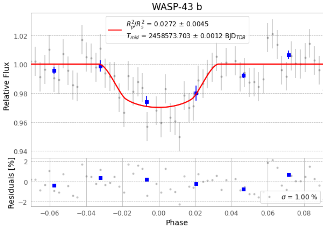
Figure 1 — FinalLightCurve_WASP-43 b_2019-03-30.png (SHA-256 6f60f85fa98da1cd...)
