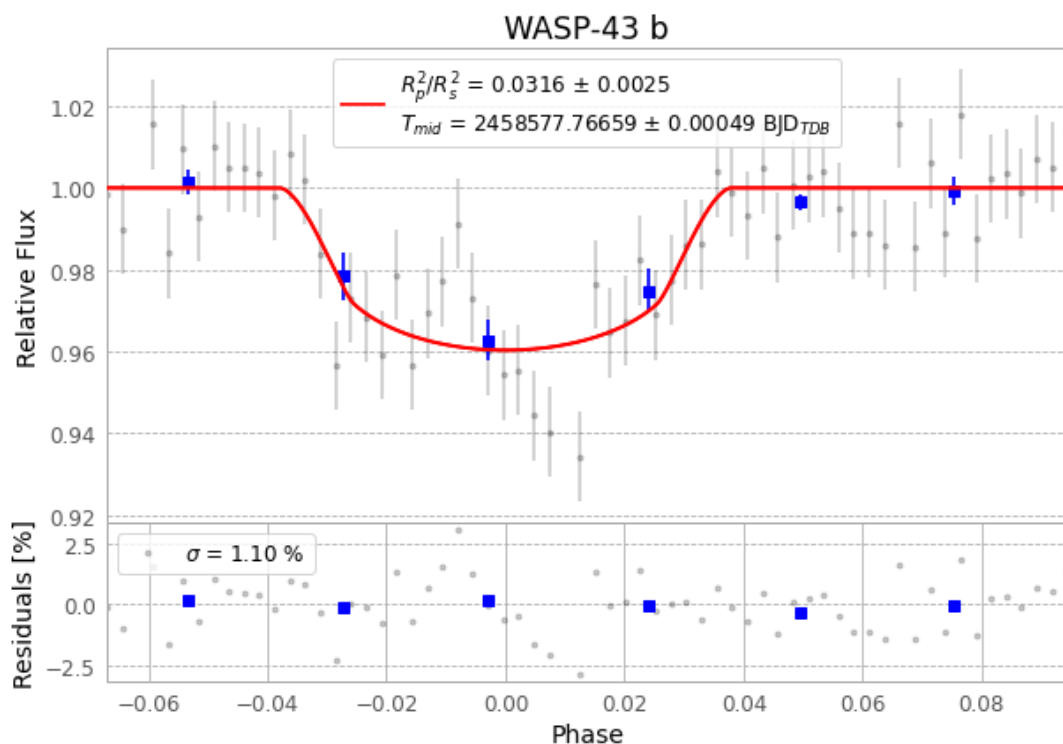
Figure 1 — FinalLightCurve_WASP-43 b_2019-04-03.png (SHA-256 18d7c4947752c8b0...)
