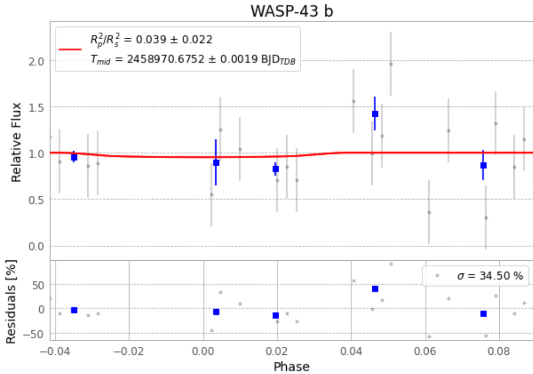
Figure 1 — FinalLightCurve_WASP-43 b_2020-04-30.png (SHA-256 27b7dd0ec94a7af6...)
