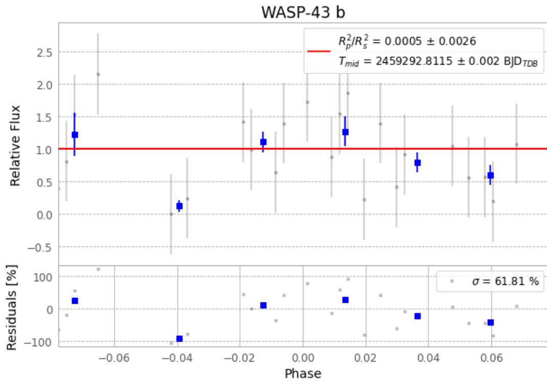
Figure 1 — FinalLightCurve_WASP-43 b_2021-03-18.png (SHA-256 5ac624d9ab1e0ca9...)
