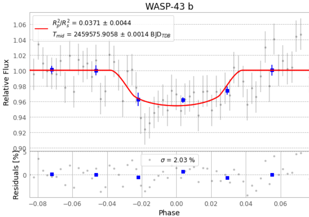
Figure 1 — FinalLightCurve_WASP-43 b_2021-12-27.png (SHA-256 f026a5bec7c1b56c...)
