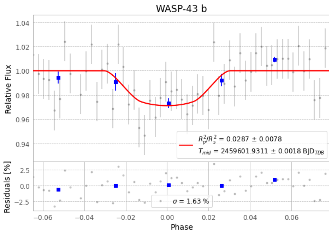
Figure 1 — FinalLightCurve_WASP-43 b_2022-01-22.png (SHA-256 67bbccee47e2e154...)
