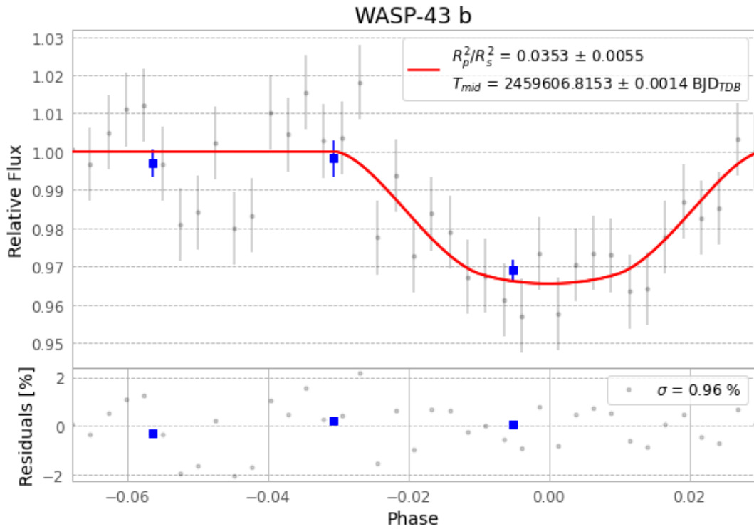
Figure 1 — FinalLightCurve_WASP-43 b_2022-01-26.png (SHA-256 f06d6f3c6c2c2872...)
