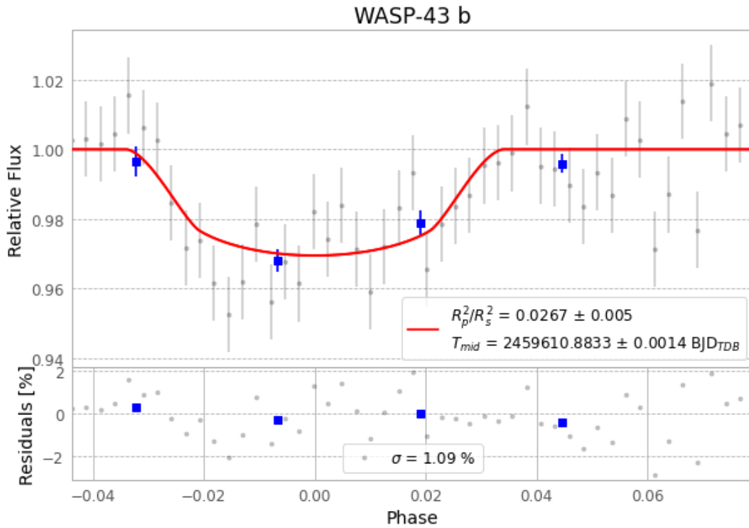
Figure 1 — FinalLightCurve_WASP-43 b_2022-01-31.png (SHA-256 e495e40d8bb38973...)
