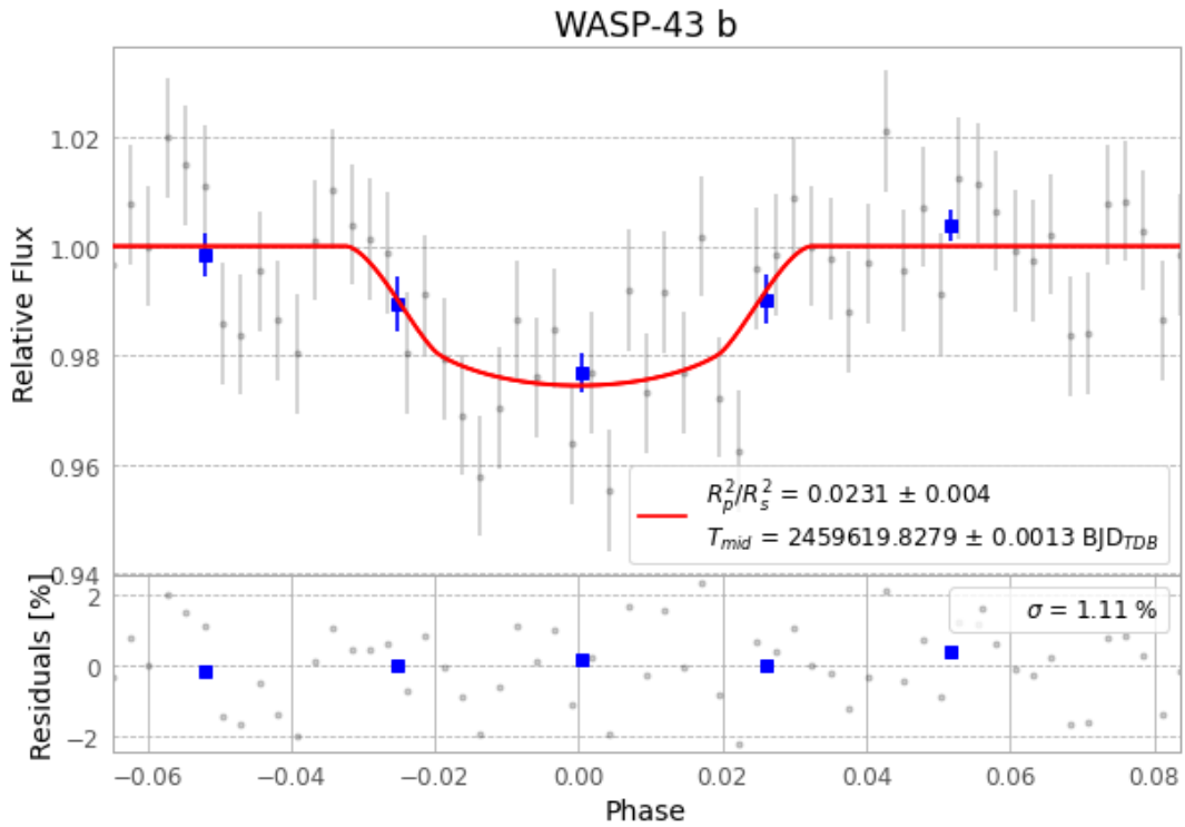
Figure 1 — FinalLightCurve_WASP-43 b_2022-02-08.png (SHA-256 5cdbbb01a0ce95ce...)
