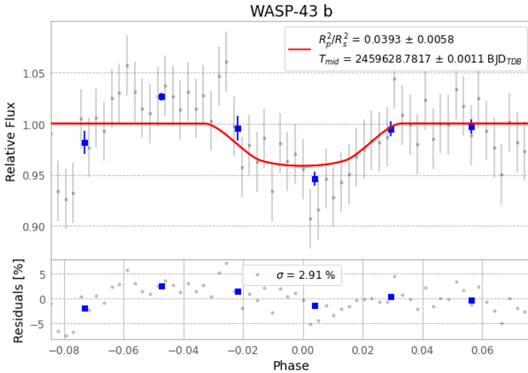
Figure 1 — FinalLightCurve_WASP-43 b_2022-02-17.png (SHA-256 84ee2f9a34254cf1...)
