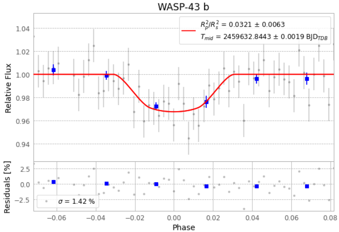
Figure 1 — FinalLightCurve_WASP-43 b_2022-02-21.png (SHA-256 28f250deb07d905f...)
