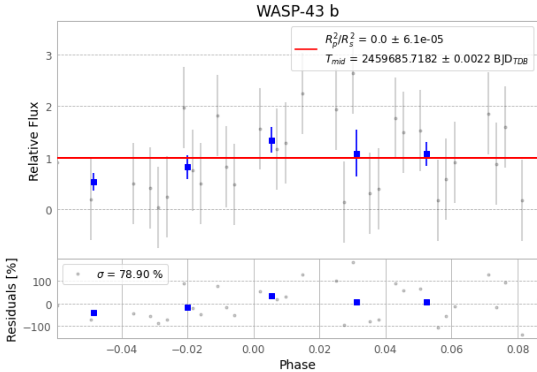
Figure 1 — FinalLightCurve_WASP-43 b_2022-04-15.png (SHA-256 ddca8af5c1c9f0fc...)
