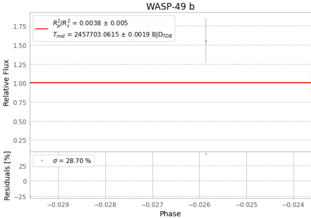
Figure 1 — FinalLightCurve_WASP-49 b_2016-11-12.png (SHA-256 73fc37fadb11673...)
