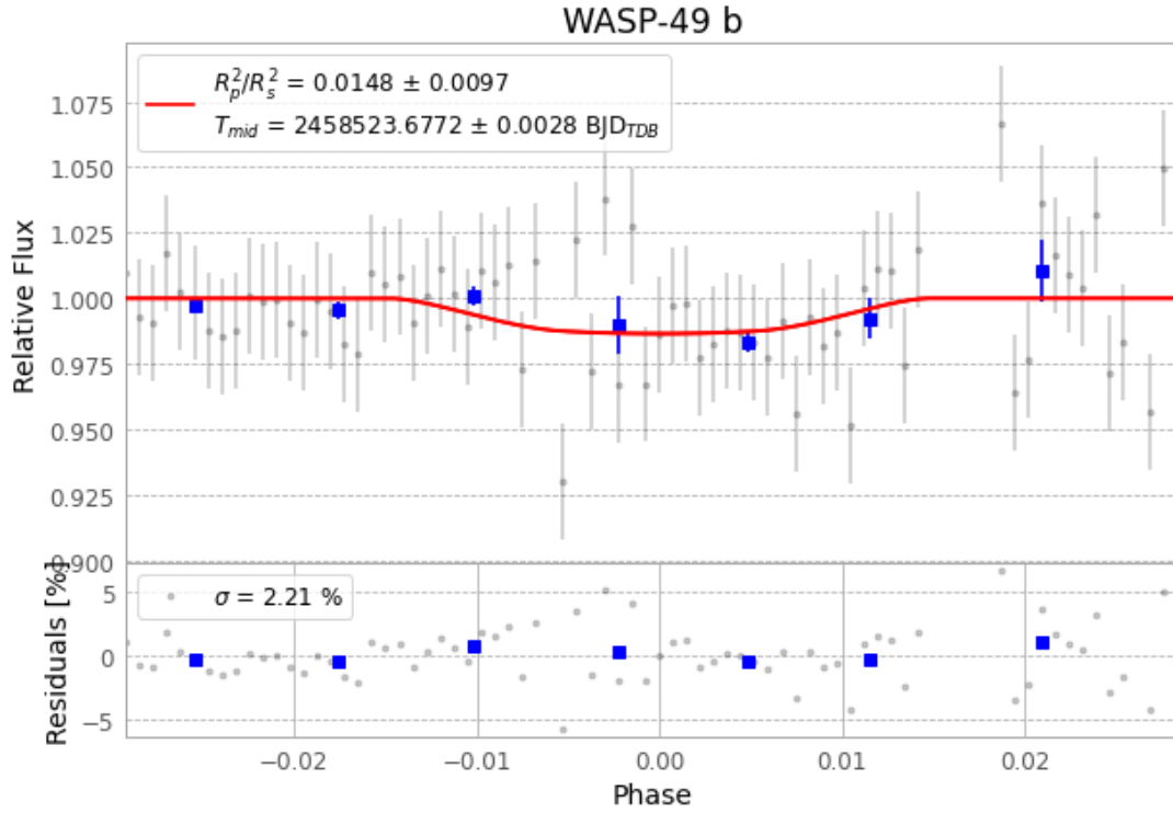
Figure 1 — FinalLightCurve_WASP-49 b_2019-02-08.png (SHA-256 c794c0c160d972da...)
