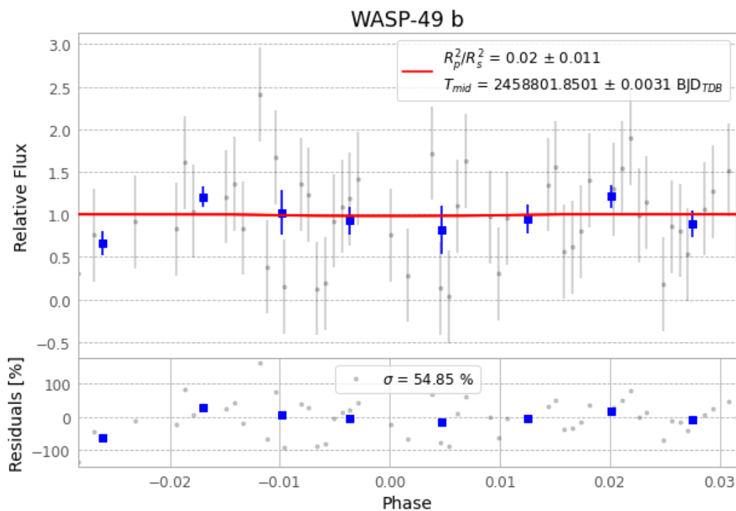
Figure 1 — FinalLightCurve_WASP-49 b_2019-11-13.png (SHA-256 10438efe87bf2d06...)
