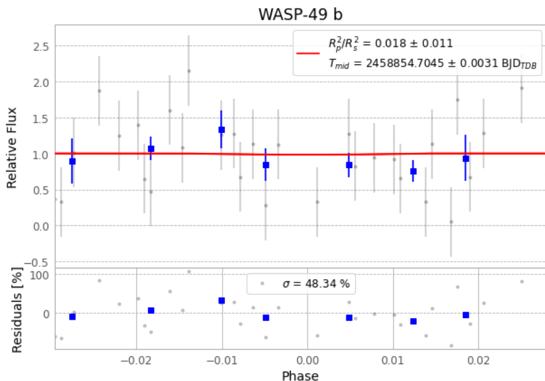
Figure 1 — FinalLightCurve_WASP-49 b_2020-01-05.png (SHA-256 71e9ee529b7c1104...)
