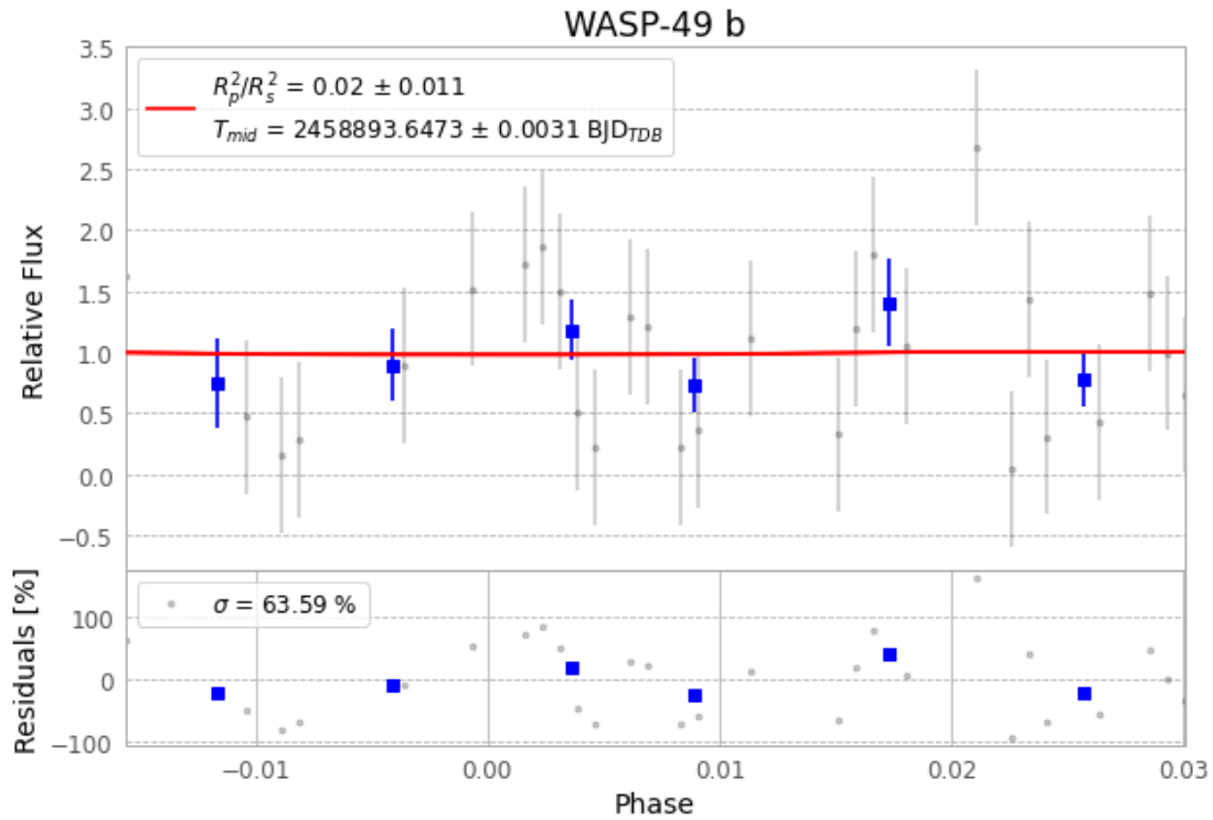
Figure 1 — FinalLightCurve_WASP-49 b_2020-02-13.png (SHA-256 39788c8793640b83...)
