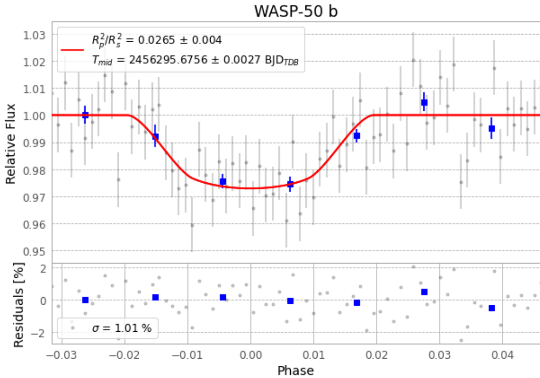
Figure 1 — FinalLightCurve_WASP-50 b_2013-01-02.png (SHA-256 3d941298044c14cf...)
