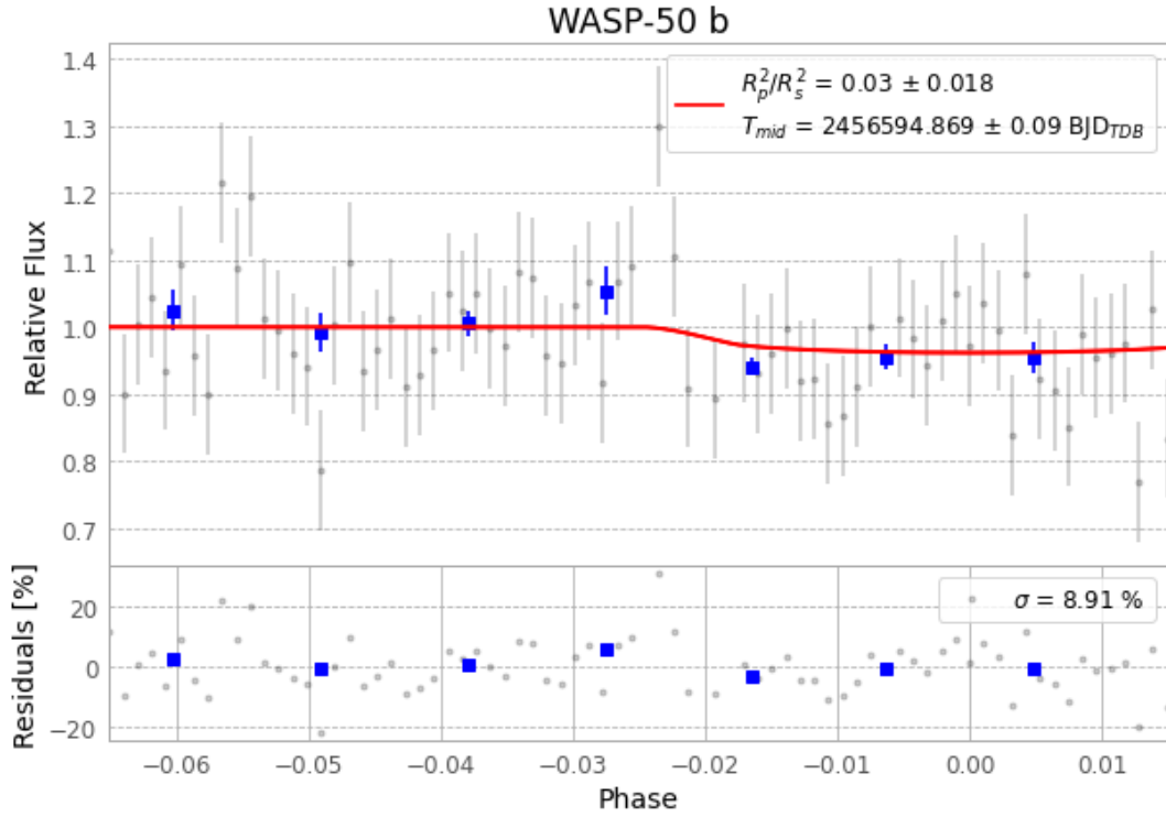
Figure 1 — FinalLightCurve_WASP-50 b_2013-10-28.png (SHA-256 1147c188021eac6e...)
