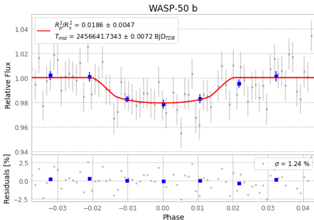
Figure 1 — FinalLightCurve_WASP-50 b_2013-12-14.png (SHA-256 795f2ecd9737f8f2...)
