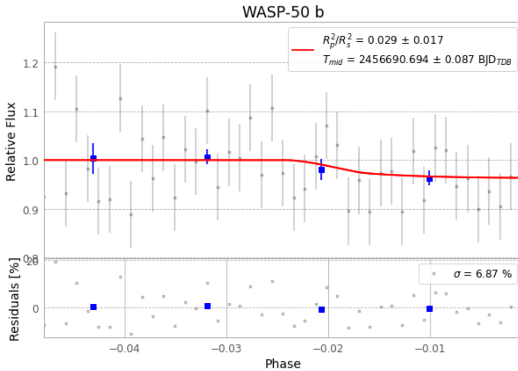
Figure 1 — FinalLightCurve_WASP-50 b_2014-02-01.png (SHA-256 8d90f7cb0f7a2513...)
