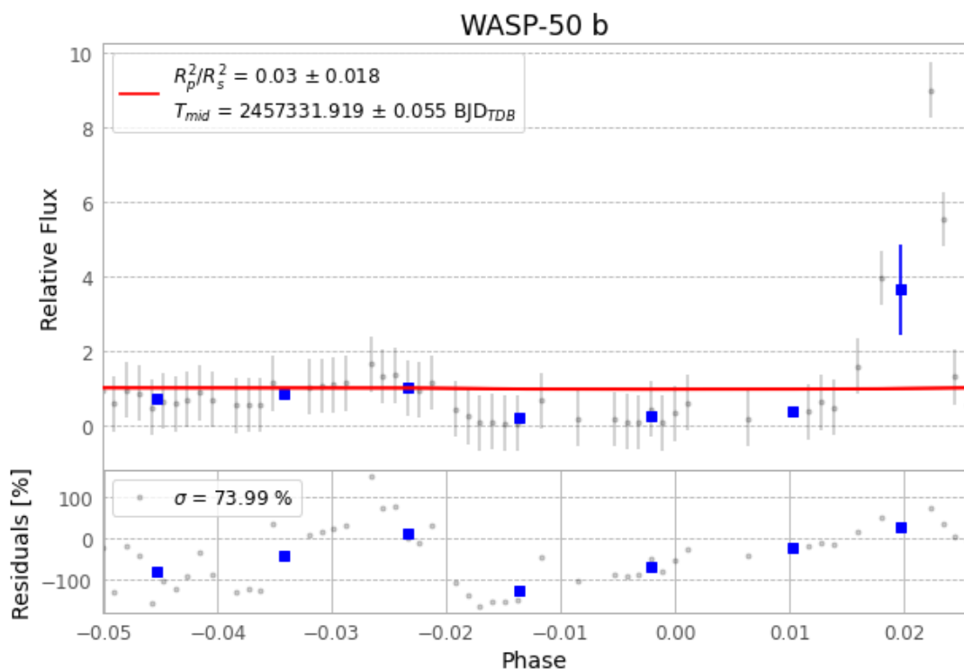
Figure 1 — FinalLightCurve_WASP-50 b_2015-11-05.png (SHA-256 6029669546e74ecc...)
