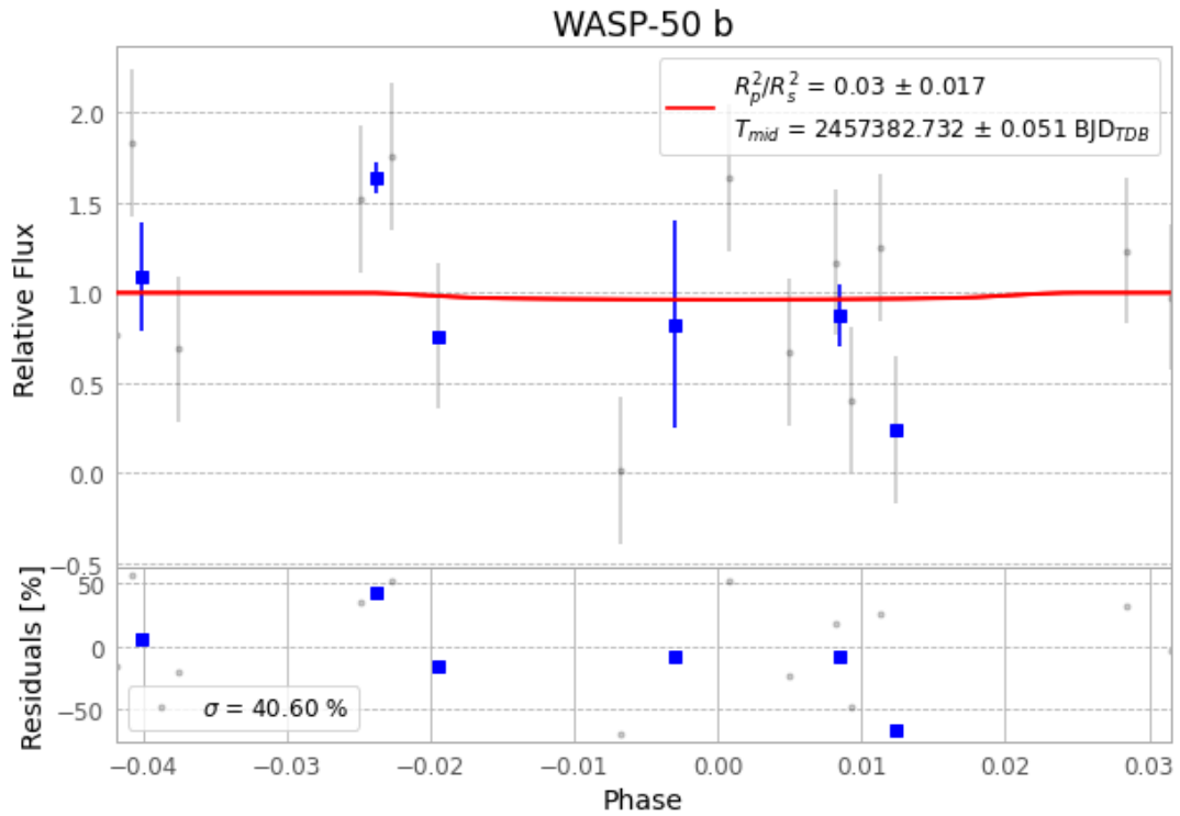
Figure 1 — FinalLightCurve_WASP-50 b_2015-12-25.png (SHA-256 a6556cbbbcd58bf0...)
