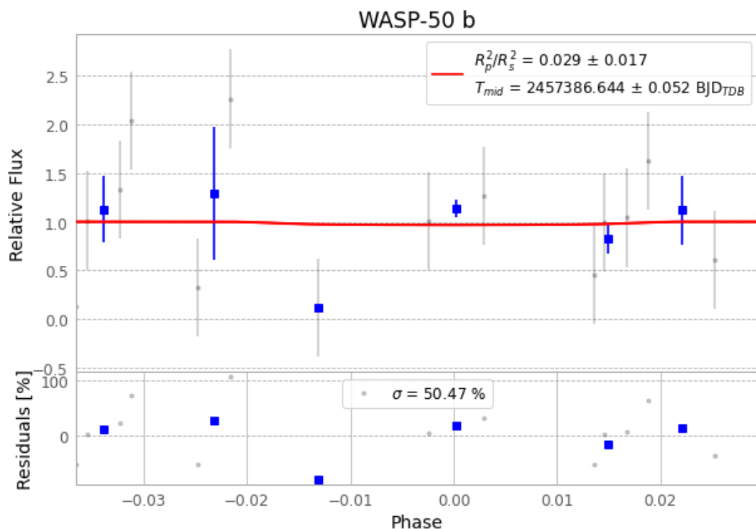
Figure 1 — FinalLightCurve_WASP-50 b_2015-12-29.png (SHA-256 978881f59aa14212...)
