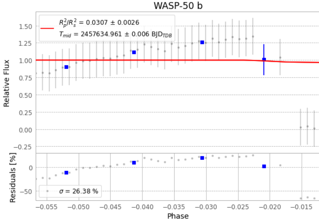
Figure 1 — FinalLightCurve_WASP-50 b_2016-09-03.png (SHA-256 3dc697bd73fa667a...)
