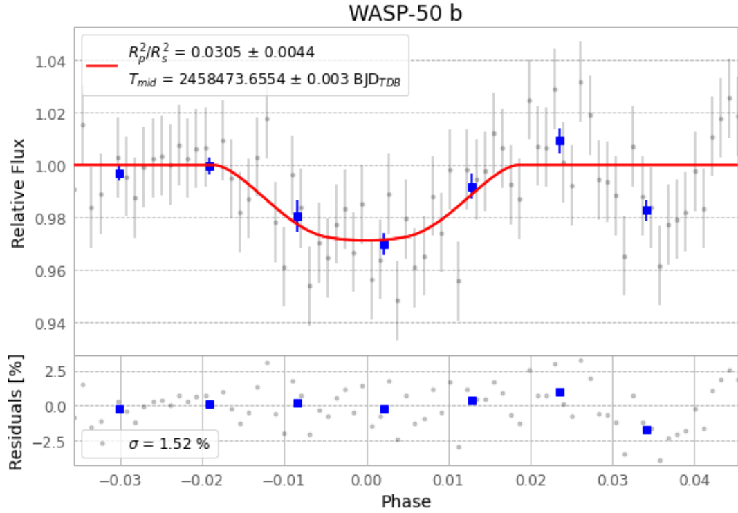
Figure 1 — FinalLightCurve_WASP-50 b_2018-12-20.png (SHA-256 7557fa1b689acad4...)
