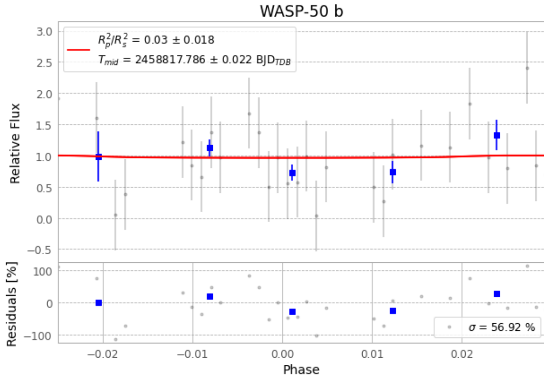
Figure 1 — FinalLightCurve_WASP-50 b_2019-11-29.png (SHA-256 e1b51f533fabe797...)
