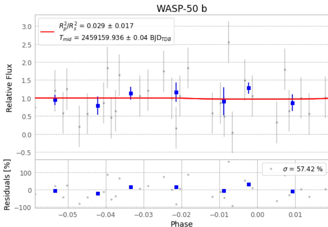
Figure 1 — FinalLightCurve_WASP-50 b_2020-11-06.png (SHA-256 44a2e9b078689166...)
