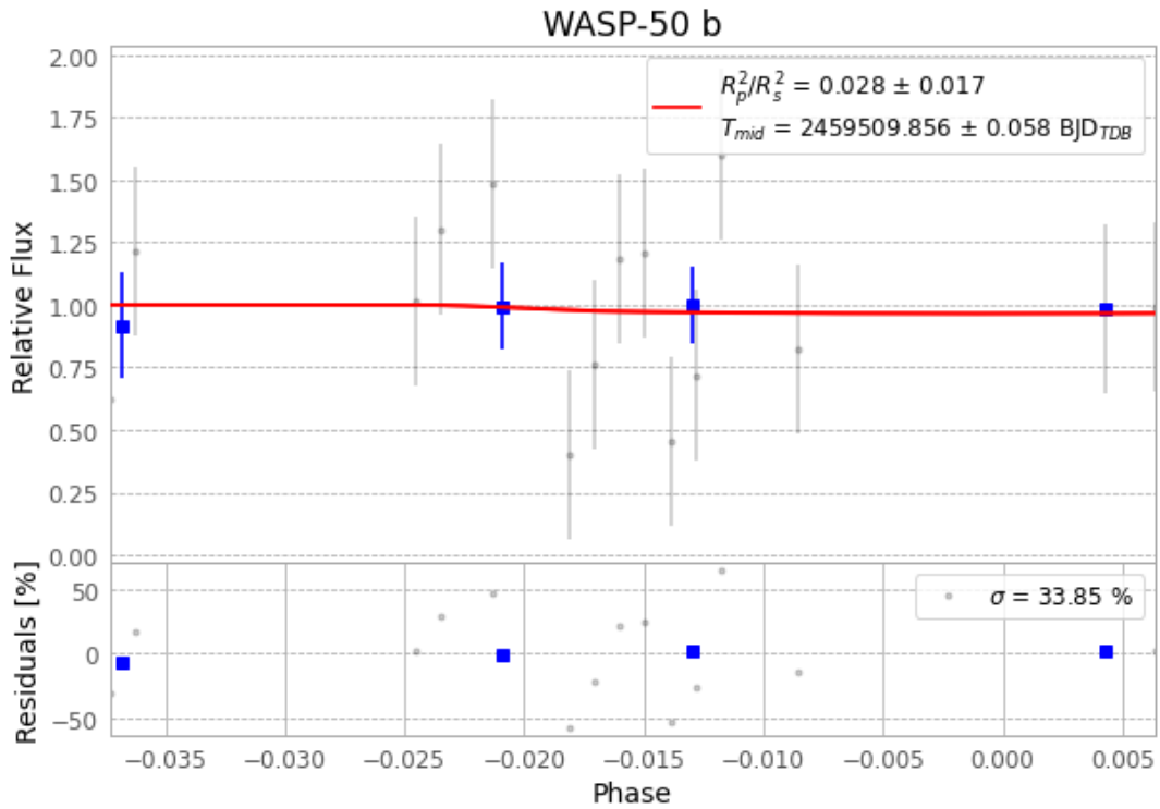
Figure 1 — FinalLightCurve_WASP-50 b_2021-10-21.png (SHA-256 75c5731dfdc5b51b...)
